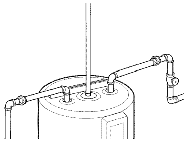
Typical horizontal piping arrangement
