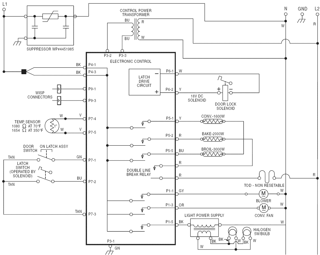
Oven schematic
