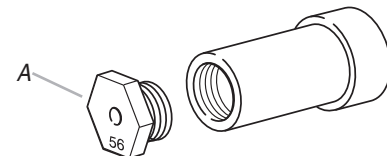
A. LP oven orifice spud stamped with "56"
