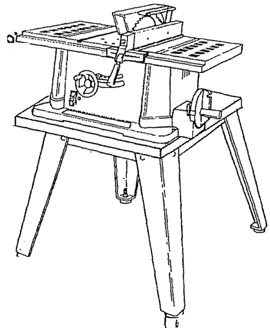
Diagram of Cabinet or Legset Mounting Holes *These holes used for legset 9-22235
