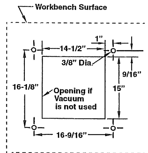
(Front of Table Saw) Diagram of Workbench Mounting Holes
