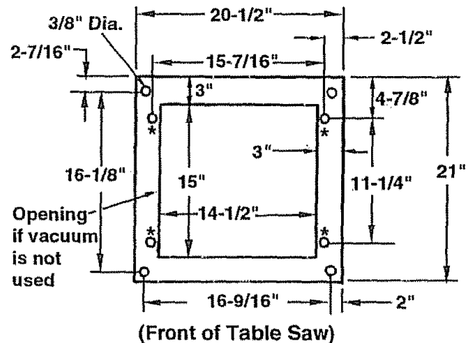
Diagram of Cabinet or Legset Mounting Holes *These holes used for legset 9-22235
