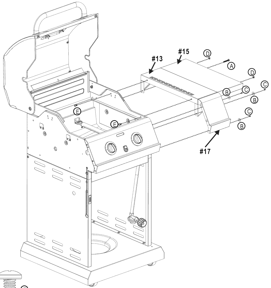
1/4-20x1/2" Screw Qty. 4 Tornillo de 1/4-20 x 1/2" Cant. 4
