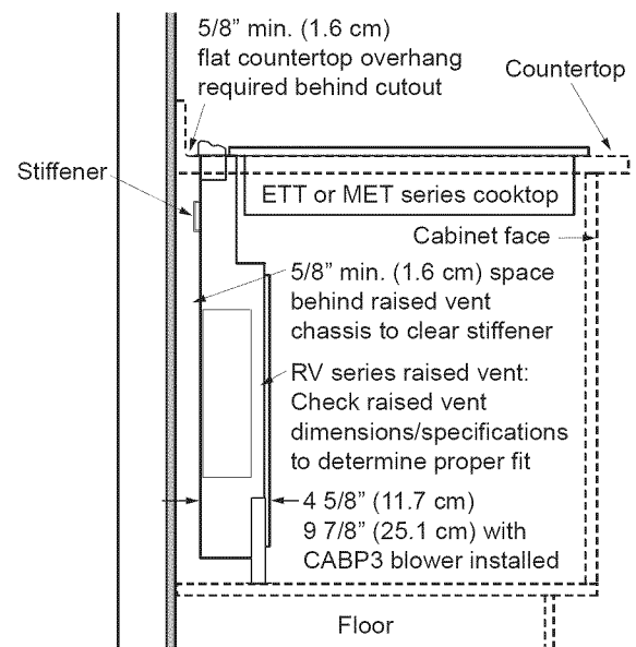
Side View: Cooktop and RV Series Raised Vent
