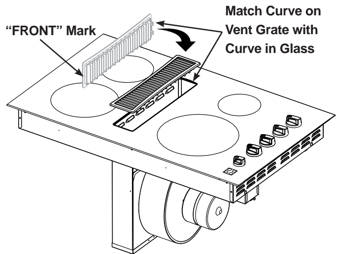
Figure 25 – INSTALL THE VENT GRATE
