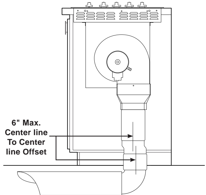
Figure 7 – DUCTWORK ALIGNMENT
