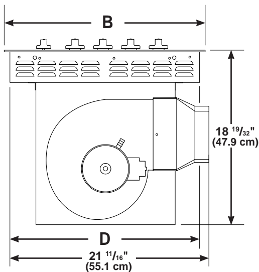
Figure 1 - PRODUCT DIMENSIONS
