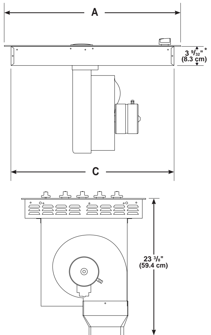
Figure 1 - PRODUCT DIMENSIONS
