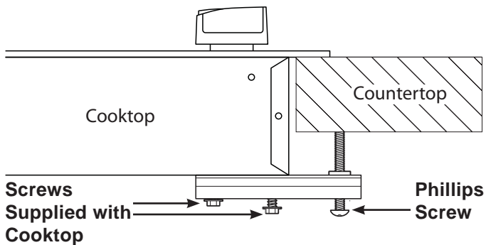
Figure 16 – SECURE COOKTOP TO COUNTERTOP
