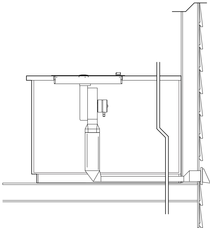
Figure 9 – DUCT ON-THE-FLOOR
