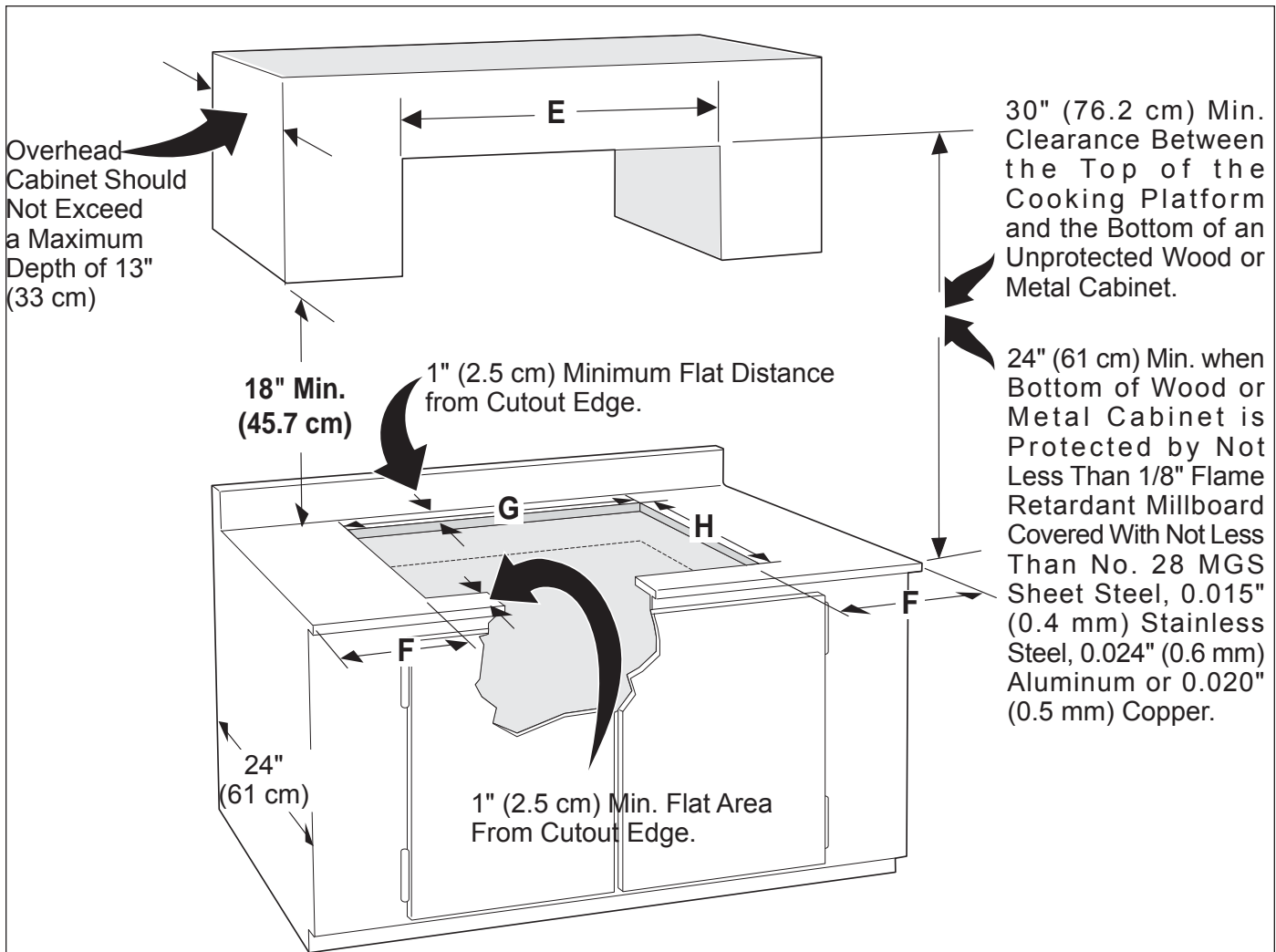
Figure 2 – CABINET DESIGN
