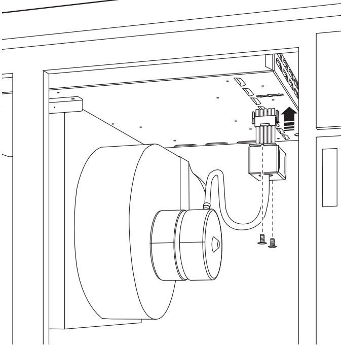
Figure 21 – CONNECT BLOWER TO COOKTOP
