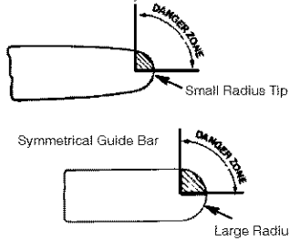
Reduced Kickback Symmetrical Guide Bar
