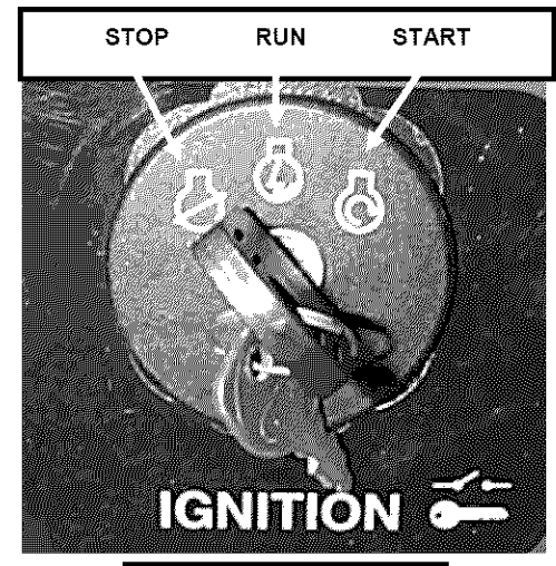
IGNITION SWITCH
