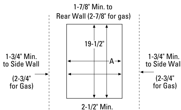
Front to Back Orientation
