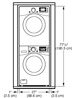
Required Dimensions for Installation With Stacking Kit
