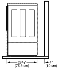
Required Dimensions for Installation With Pedestal
