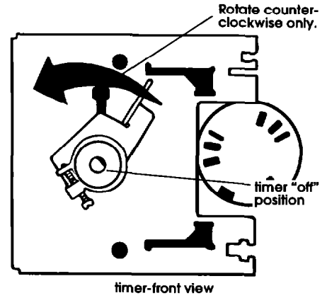
timer-front view
