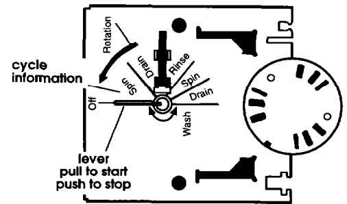
timer-rear view
