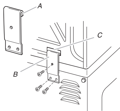
A. Hooked end B. Stack bracket C. Slot in dryer back
