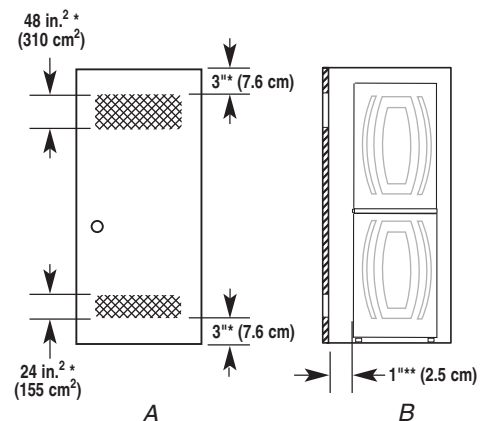
A. Closet door minimum ventilation openings B. Side view of stacked washer and dryer
