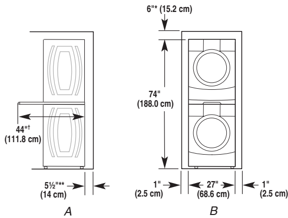
A. Side view of stacked washer and dryer B. Front view of stacked washer and dryer
