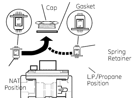
Pressure Regulator
