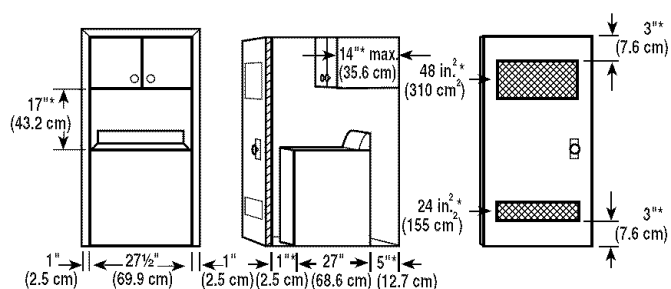
A. Front view B. Side view C. Closet door with vents
