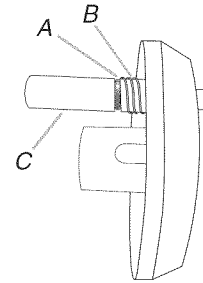
A. Retaining clip B. Spring C. LP gas igniter
